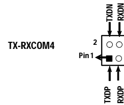
RS422/485 Header
